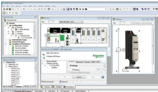
CANopen configuration in Unity Pro with BMECXM0100
