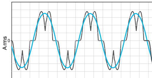
— Harmonic level without harmonic filtering ( \text{THDI} \sim 48\% ) — Harmonic level with harmonic filtering ( \text{THDI} \leq 5\% )
